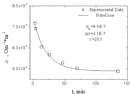
FIGURE 2 Measured (symbols) and fitted (line) dependencies of dielectric conductivity \sigma of LC cell based on rubbed PI substrates on the time passed after the sample filling with LC 5CB.
