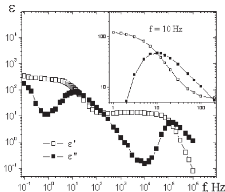
FIGURE 1 The frequency dependencies of real \epsilon' and imaginary \epsilon'' parts of dielectric permittivity for 5CB layer aligned on rubbed PI substrates.
